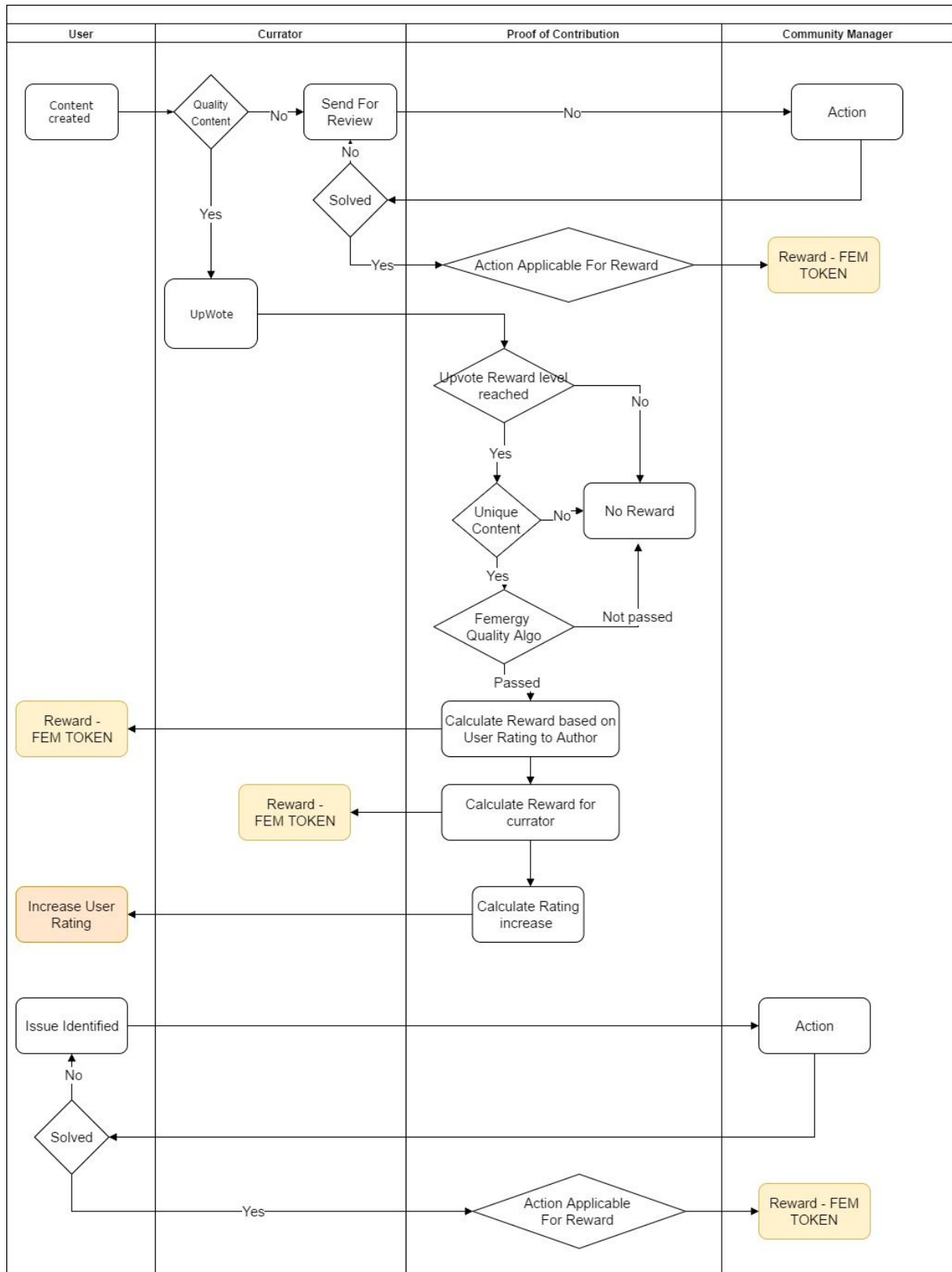
Figure 4. Proof of Contribution detailed workflow
